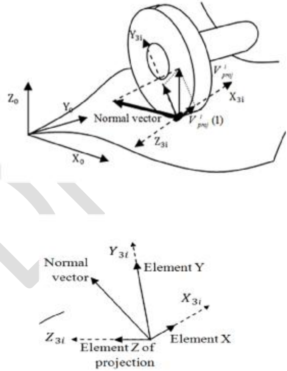
Fig. 7. Representation of the normal vector in the coordinate system X_{3i}Y_{3i}Z_{3i}
