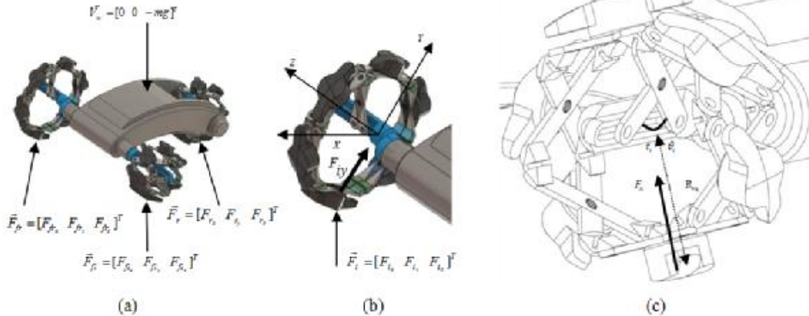
Fig. 9. Contact forces of the wheels at contact points
