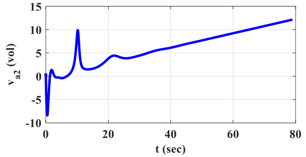
Fig. 7: The time history of the second actuator output
