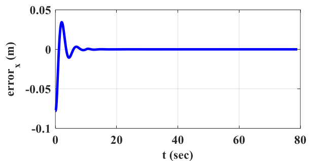
Fig. 4: The x component of the reference trajectory tracking error
