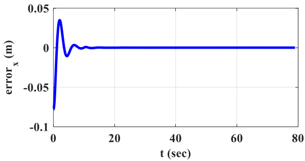
Fig. 13: The x component of the reference trajectory tracking error considering disturbed input
