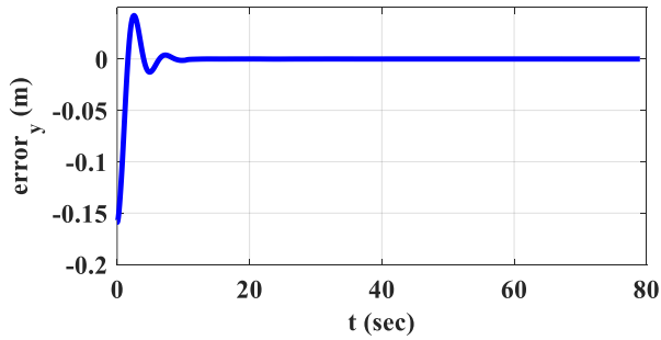
Fig. 5: The y component of the reference trajectory tracking error
