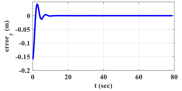
Figure 15. The y component of the reference trajectory tracking error considering disturbed input
