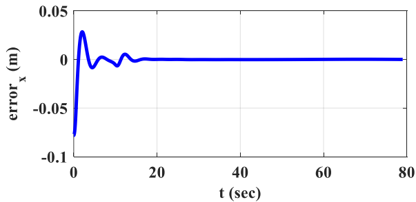
Figure 20. The x component of the reference trajectory tracking error considering uncertainty
