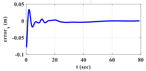
Figure 16. The x component of the reference trajectory tracking error considering step-shape disturbed input
