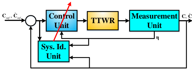
Fig. 2: The control schematic of the TTWR system
