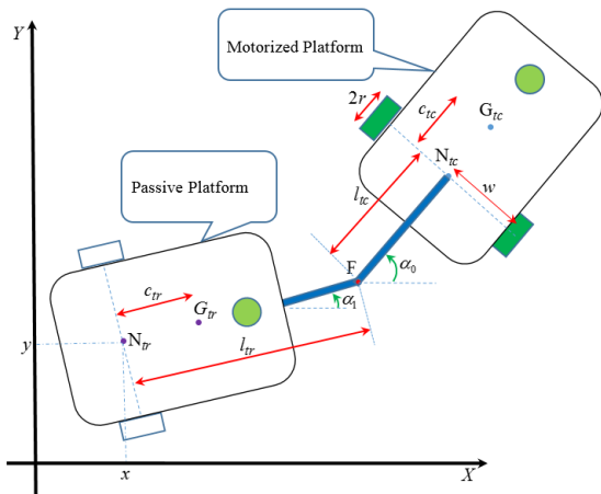
Fig. 1: The considered tractor-trailer wheeled robot system
