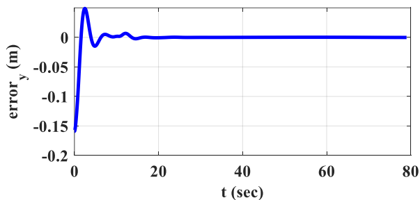
Figure 21. The y component of the reference trajectory tracking error considering uncertainty
