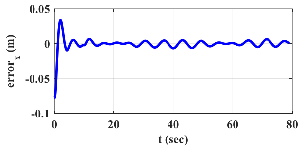
Figure 18. The x component of the reference trajectory tracking error considering sin-shape disturbed input
