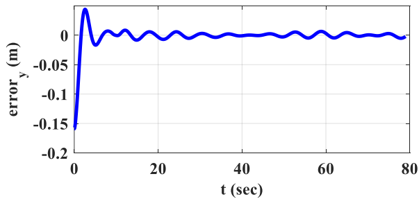
Figure 19. The y component of the reference trajectory tracking error considering sin-shape disturbed input
