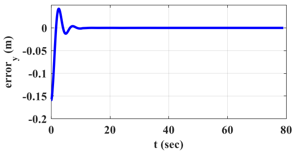
Fig. 14: The y component of the reference trajectory tracking error considering disturbed input
