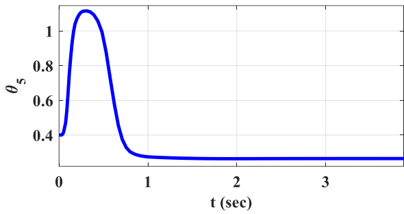
Fig. 12: The \theta_5 convergence time history
